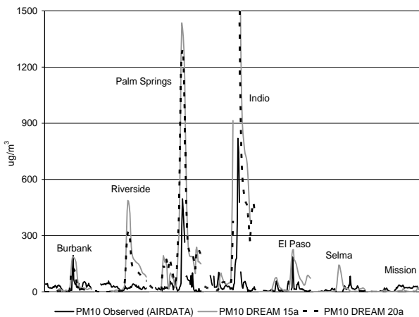
Figure 1. Modelled and observed PM 10 concentrations at seven AIRNow stations across the southwest for January 4-6, 2007.
