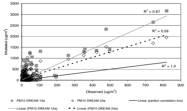
Figure 2. Magnitude correlation for seven sites during the Jan 4-6, 2007 event (N = 443).
