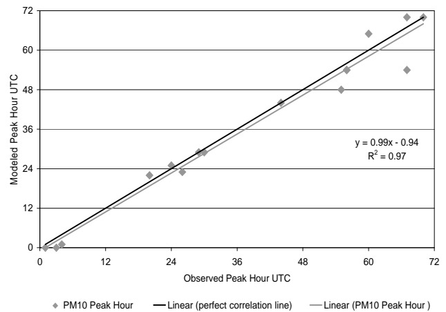
Figure 6. Timing correlation, February 23-25, 2007 event (N=16 peak hours).
