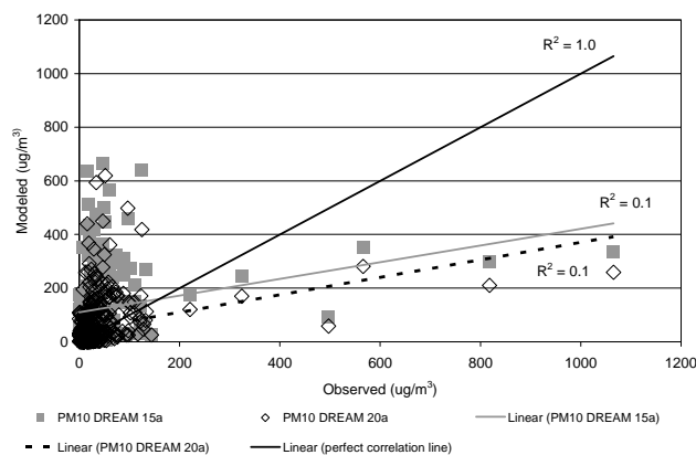
Figure 5. Magnitude correlation between observed and modelled data, February 23-25, 2007 event.
