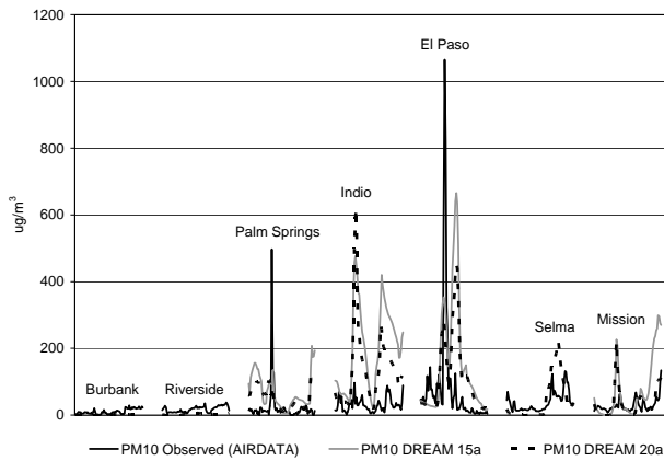
Figure 4. The February 23-25, 2007 dust episode, seven sites located in the model domain.
