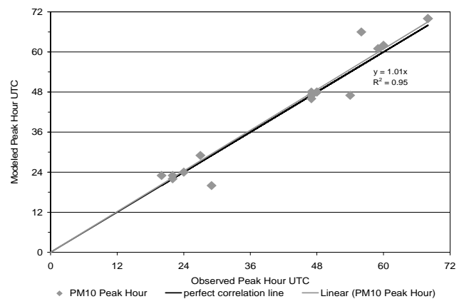
Figure 3. Timing Correlation (N=18 peak hours, seven sites) for the Jan 4-6, 2007 dust event.
